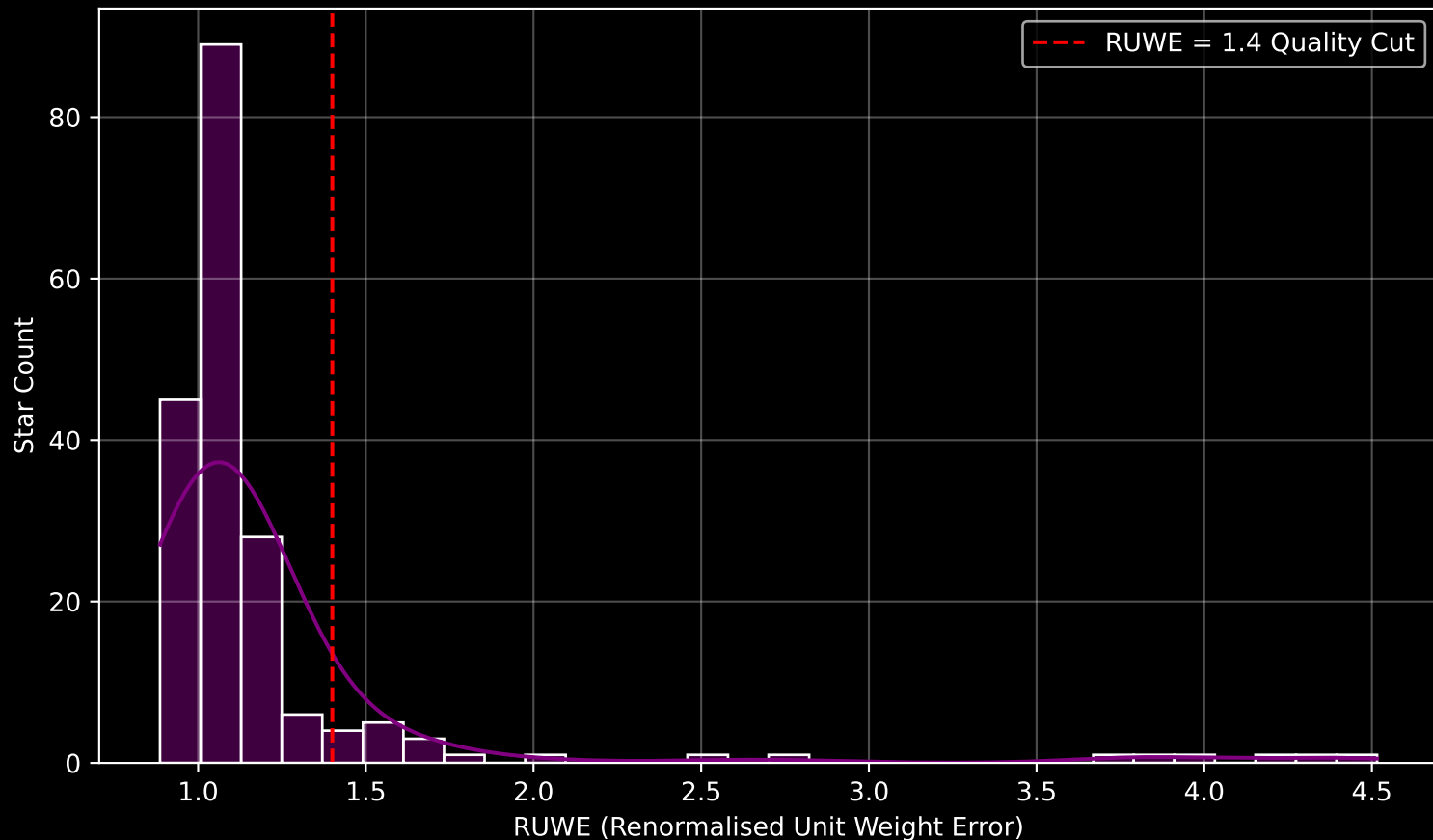
GAPOGEE DR17 Field [K2_C4_179-25_btx] RUWE Distribution (n= 190)
