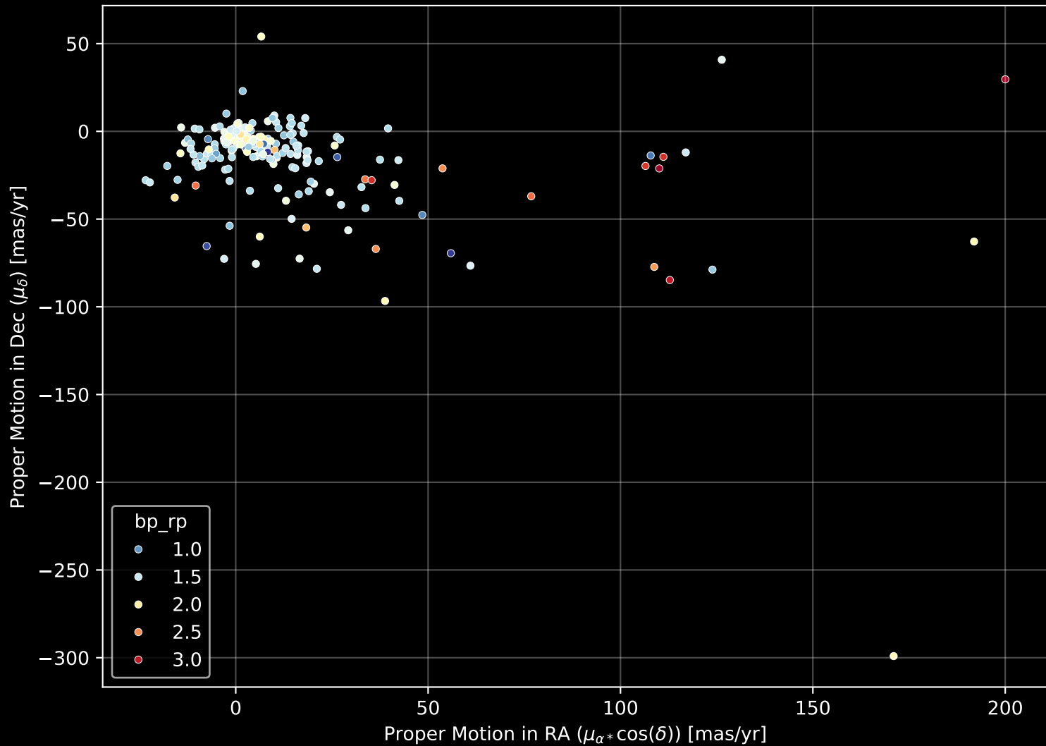
APOGEE DR17 Field: [K2_C4_179-25_btx] Proper Motion Diagram (n= 199)
