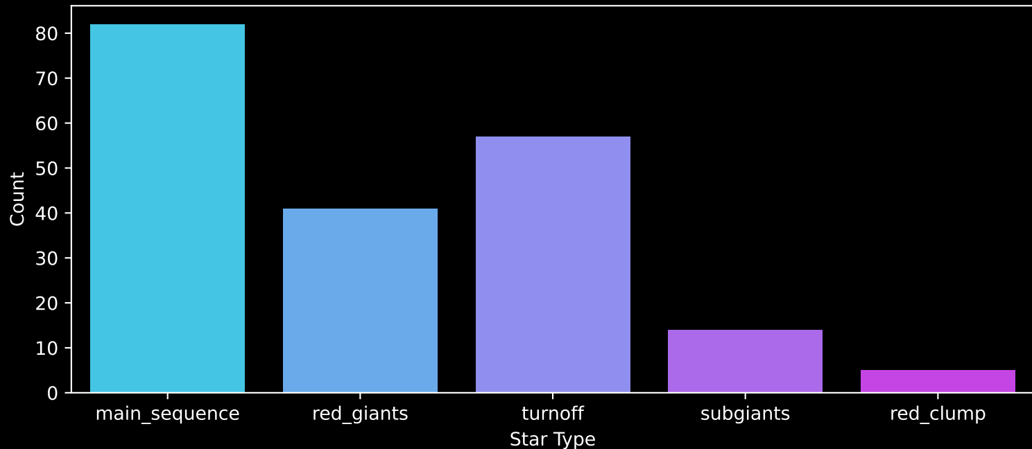
APOGEE DR17 Field: [K2_C4_179-25_btx] Count plot of Star Type
