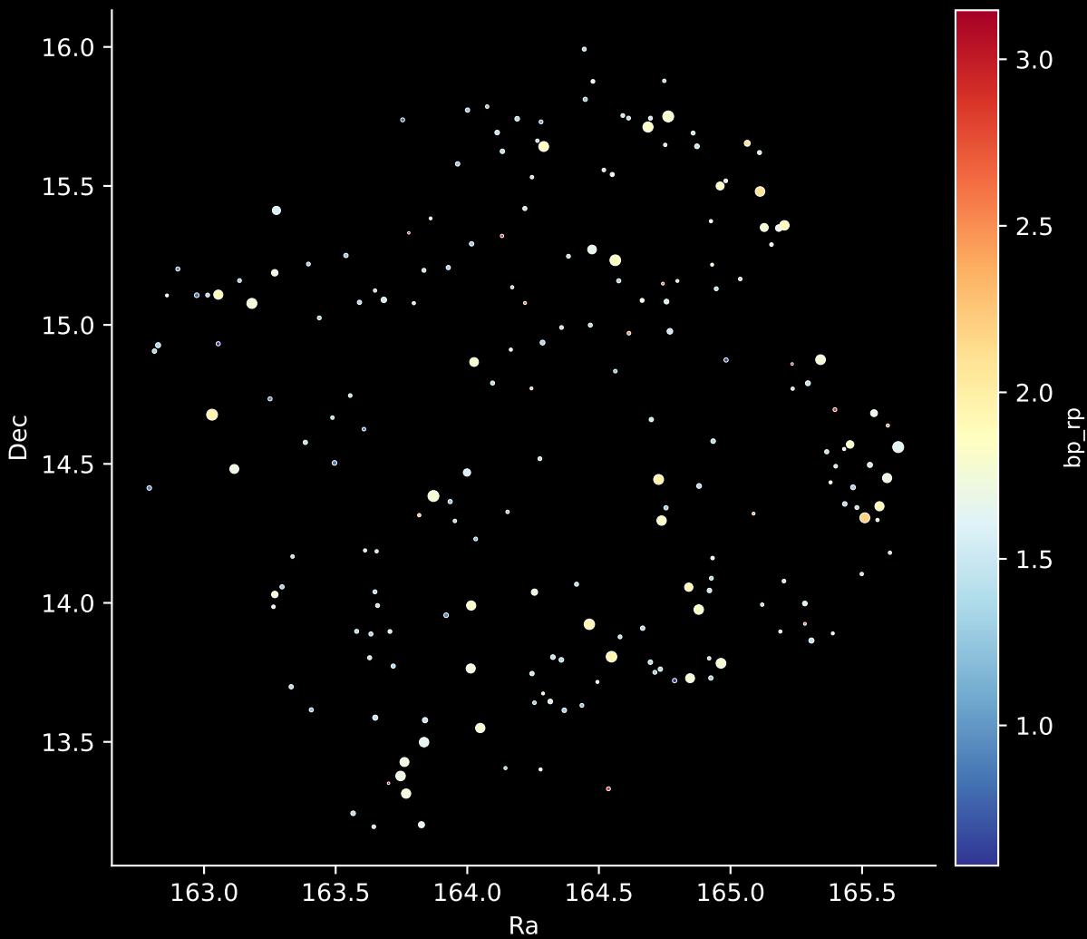
APOGEE DR17 Field: [K2_C4_179-25_btx] Stars: 199
