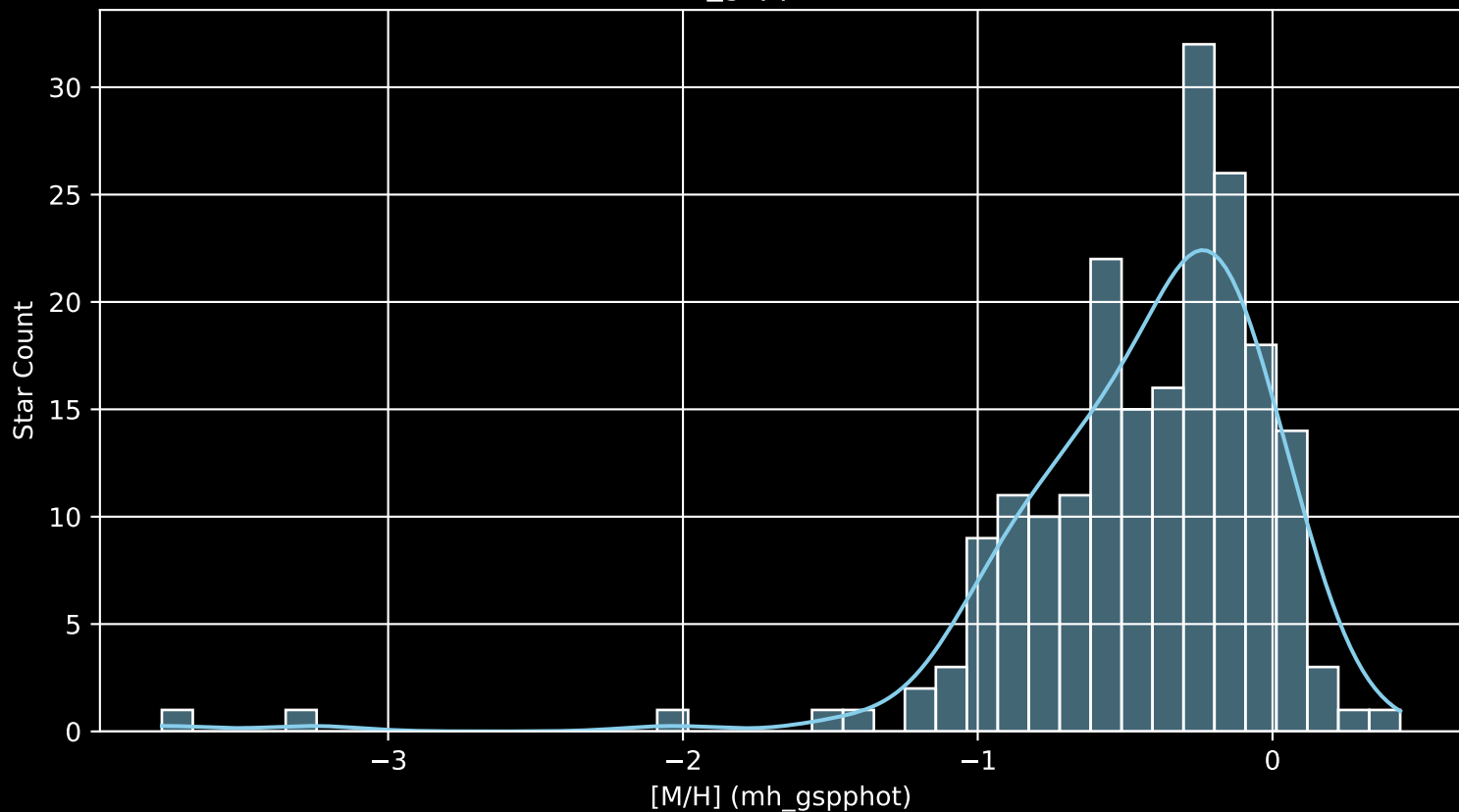
APOGEE DR17 Field: [K2_C4_179-25_btx [M/H] (mh_gspphot) (n= 199)
