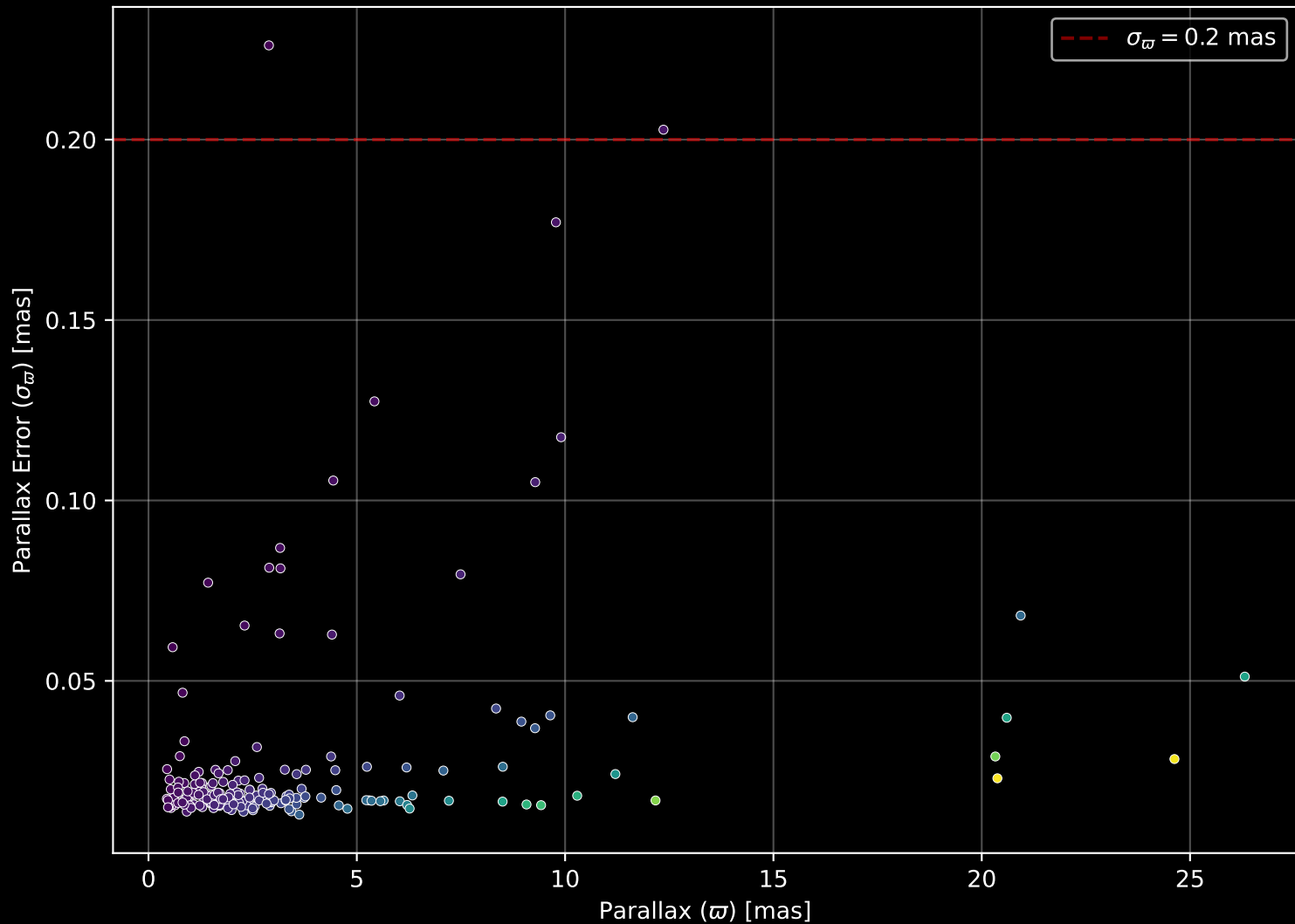
APOGEE DR17 Field: [K2_C4_179-25_btx] Parallax Quality (n= 199)
