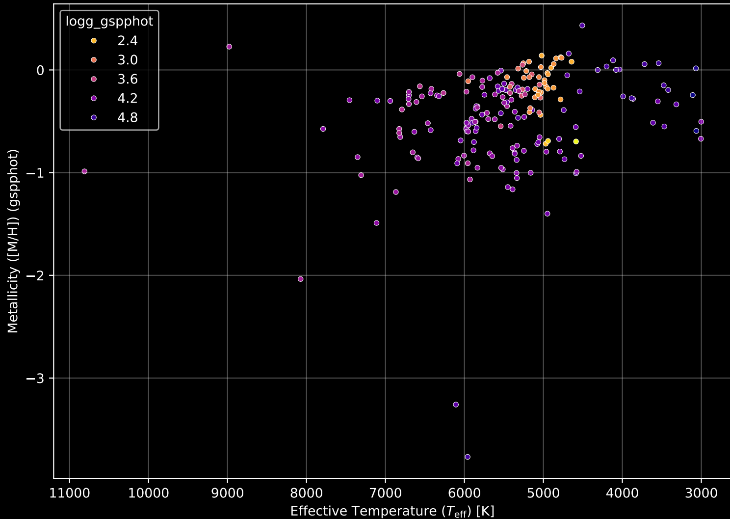
APOGEE DR17 Field: [K2_C4_179-25_btx] Stellar Population Parameters (n= 199)
